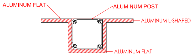
SECTION C-C
