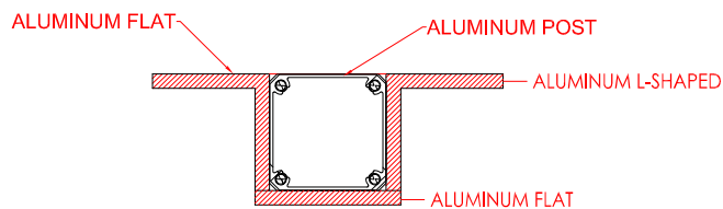
SECTION C-C
