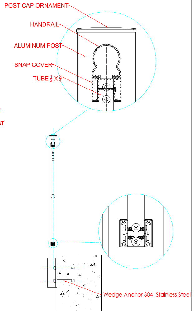
SECTION B-B
