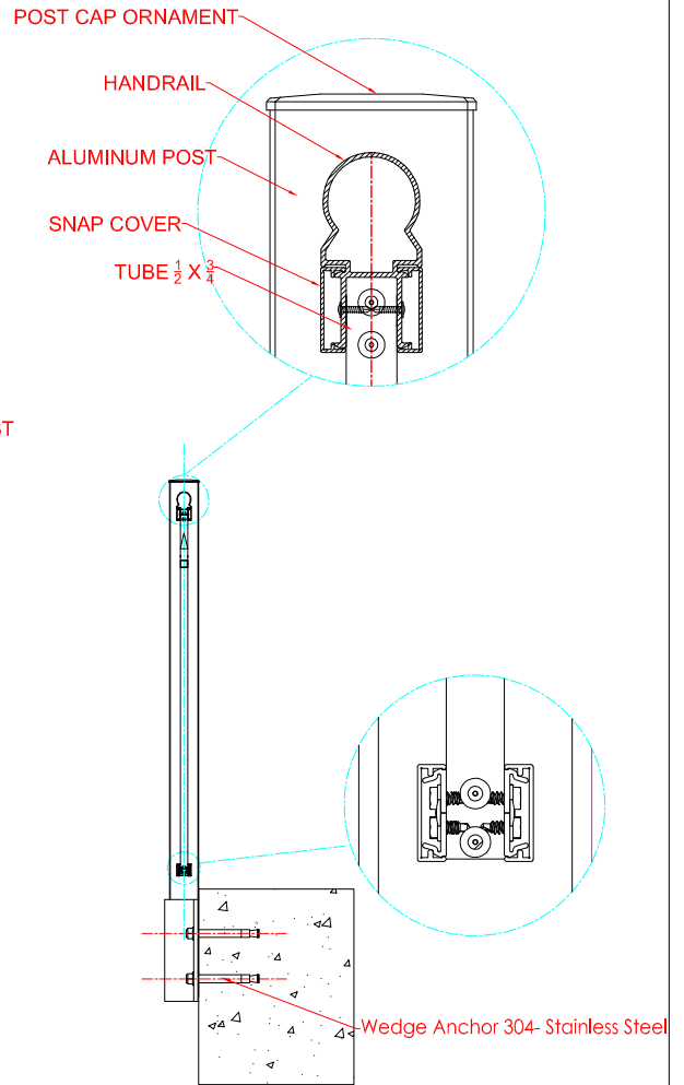
SECTION B-B
