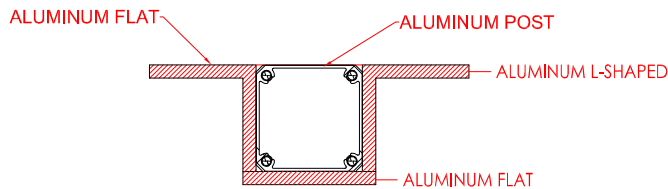
SECTION C-C
