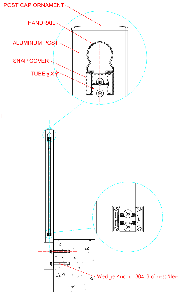
SECTION B-B
