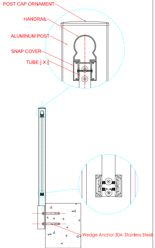
SECTION B-B
